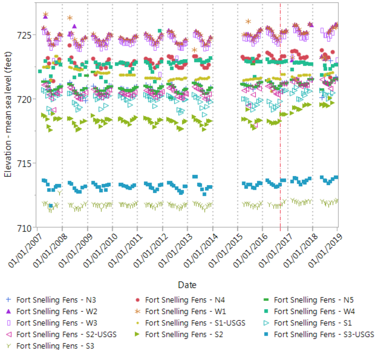
Figure 3. Water level elevation for the Fort Snelling fen wells. At well S3-USGS, when the water was overflowing, the elevation of the top of the pipe (Historical - 713.97 and 2016 – 714.18) was recorded. See individual well graphs in Appendix 3.
