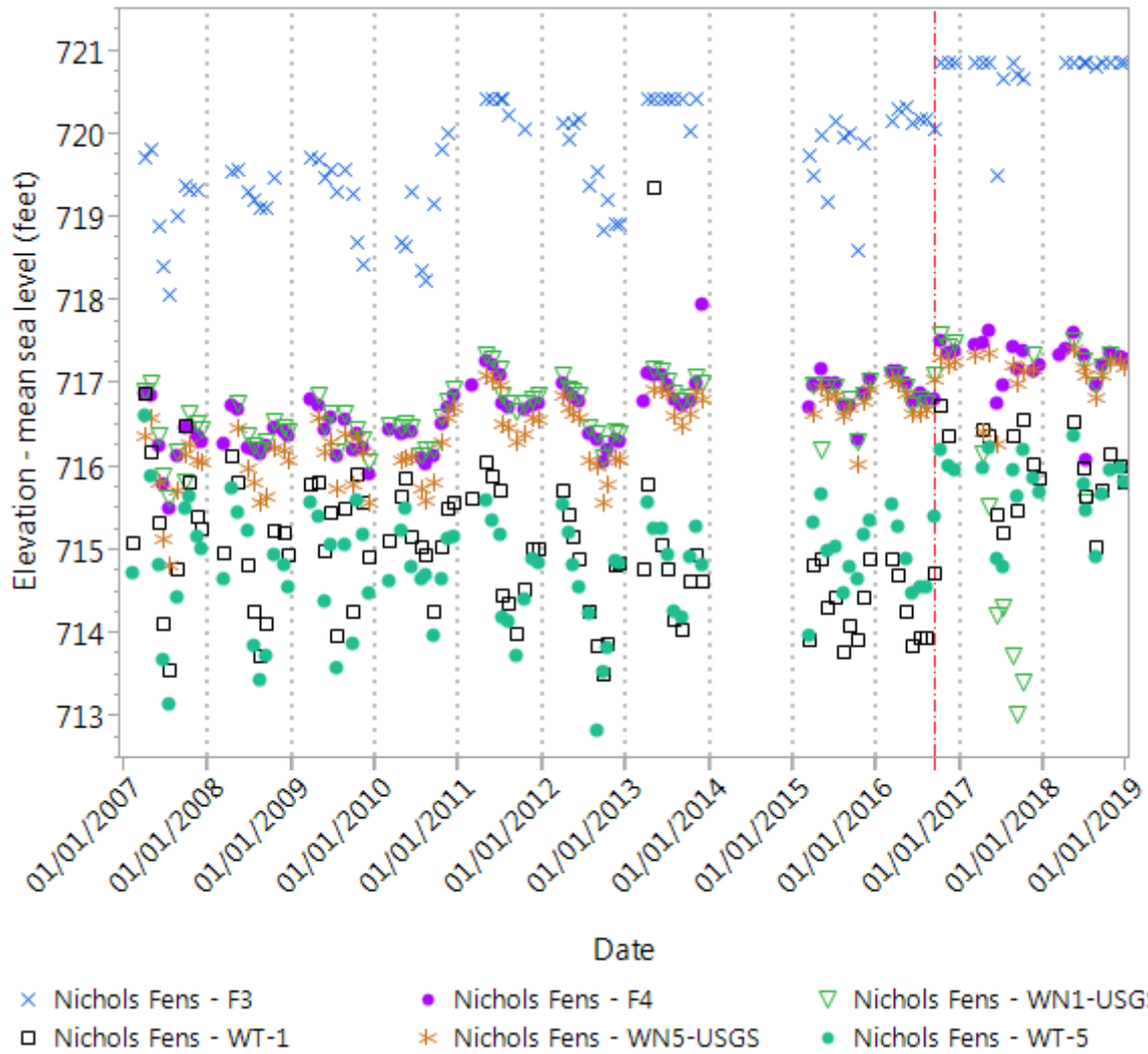
Figure 5. Water level elevation for the Nichols Fen wells (set 2 of 3). At well F3 and WT-1, the water was often overflowing and the elevation of the top of the pipe (F3: Historical - 720.43 and 2016 – 720.88; WT-1: Historical - 719.37 and 721.25) was recorded. See individual well graphs in Appendix 3.
