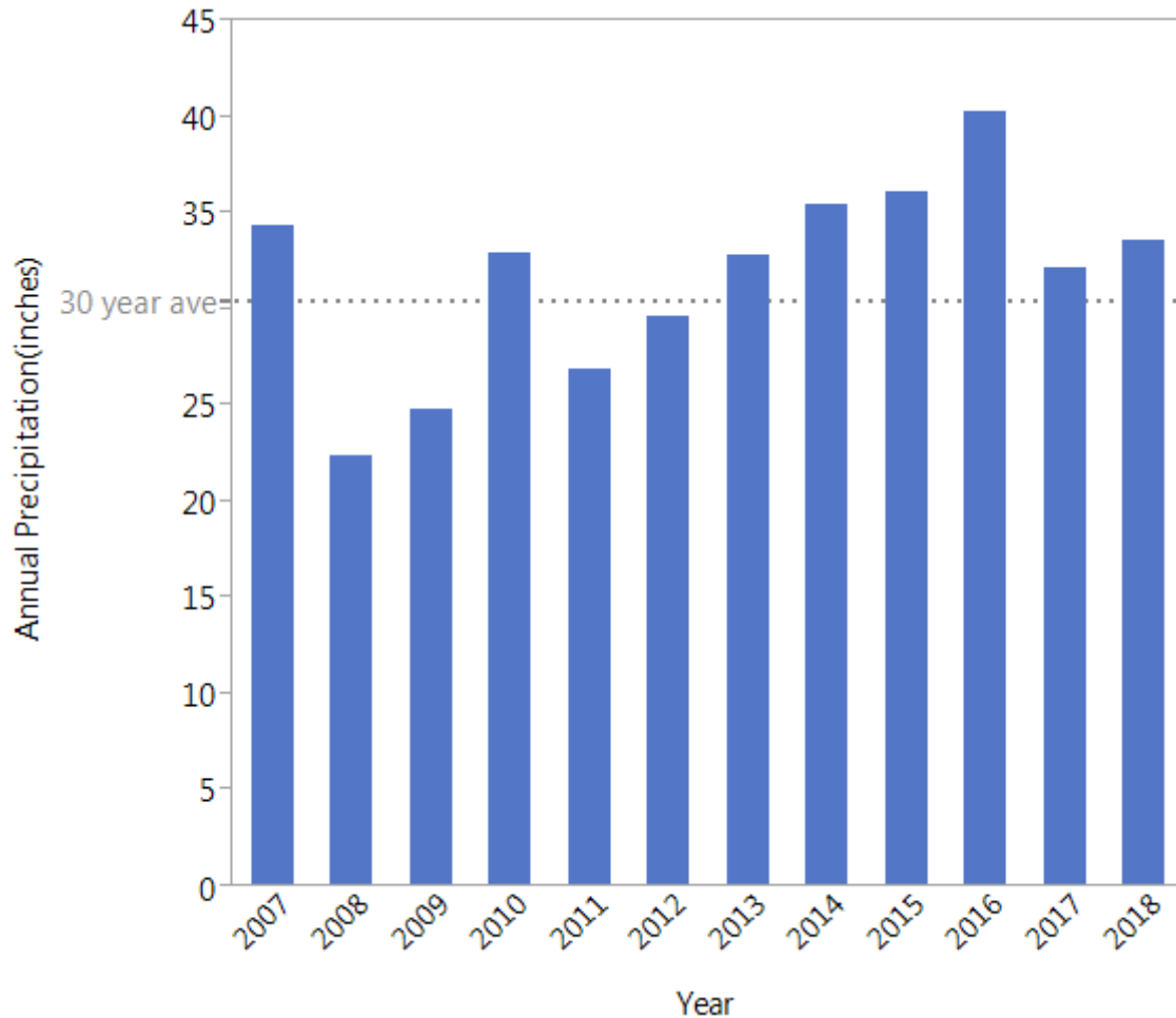
Figure 1. Total rainfall (inches) from 2007-2018 at Minneapolis/St. Paul weather station, data courtesy of the MNDNR. Gray dotted line indicates the 30 year (1988-2017) total annual average precipitation of 30.5 inches.
