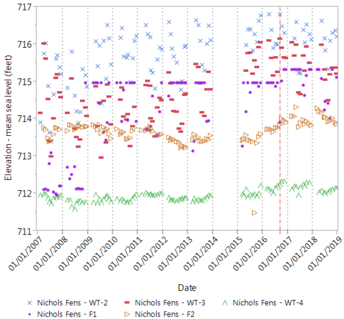
Figure 6. Water level elevation for the Nichols Fen wells (set 3 of 3). At well F1, the water was often overflowing and the elevation of the top of the pipe (Historical - 714.97 and 2016 – 715.32) was recorded. See individual well graphs in Appendix 3.
