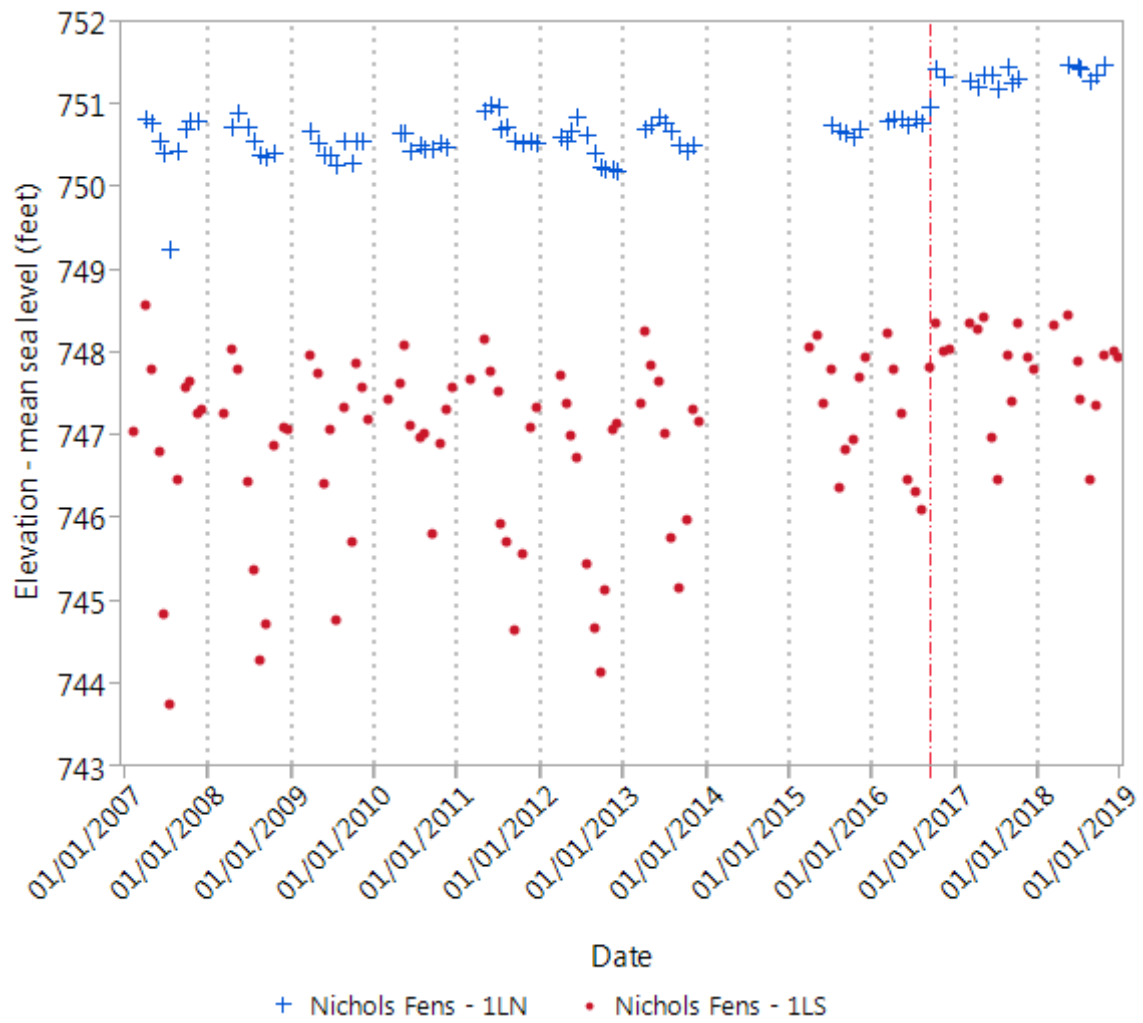
Figure 4. Water level elevation for the Nichols Fen wells (set 1 of 3).
