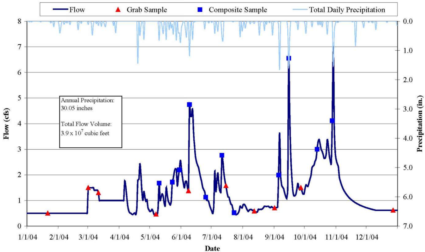
Silver Creek 2004 Hydrograph, Precipitation and Sampling Information
