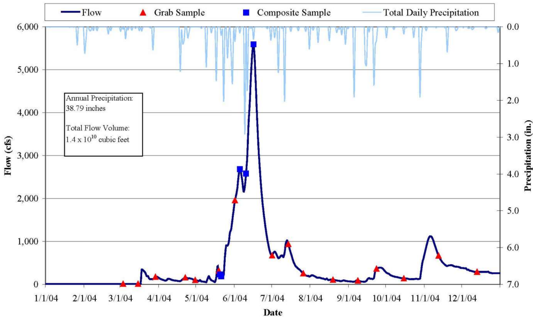
South Fork Crow River 2004 Hydrograph, Precipitation and Sampling Information
