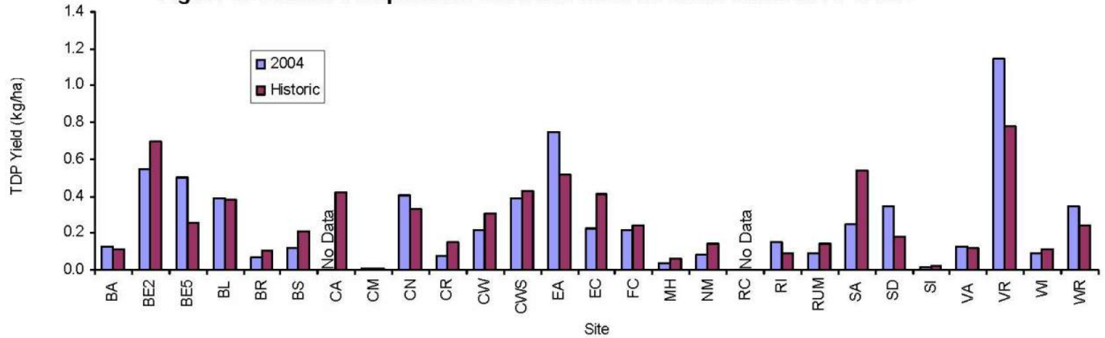
Figure 5. Stream Comparison: 2004 and Historic Mean Watershed Yields
