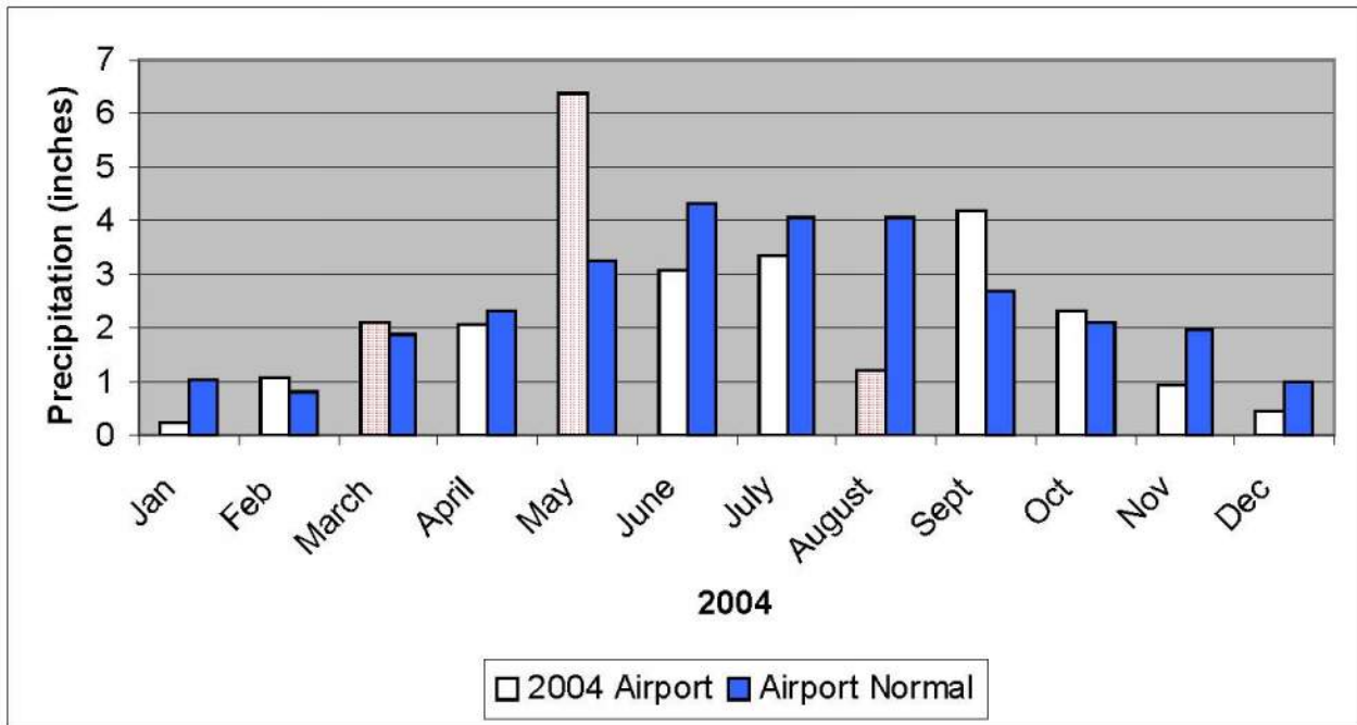
Figure 2. 2004 and Normal Monthly Precipitation at Minneapolis-St. Paul Airport
