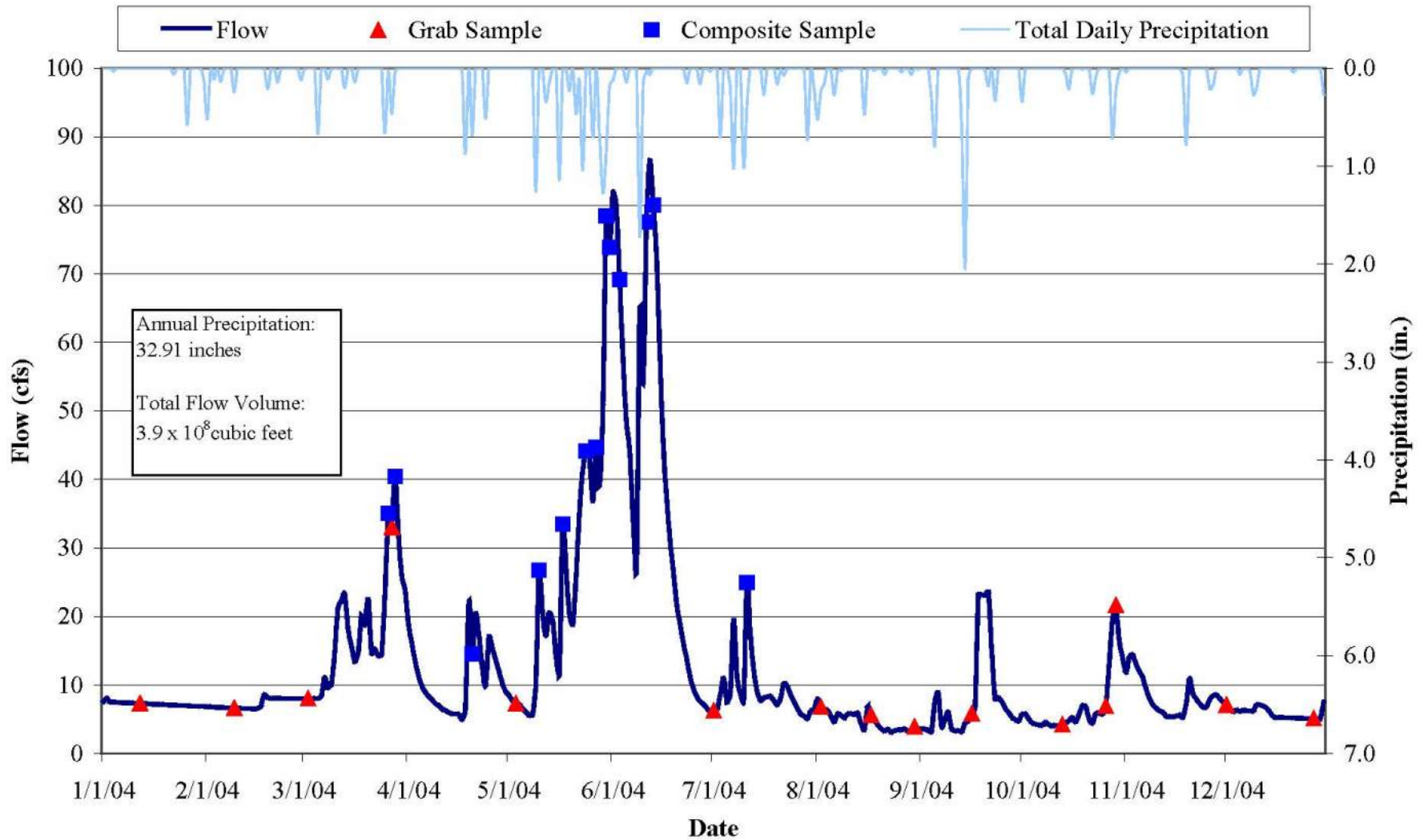
Credit River 2004 Hydrograph, Precipitation and Sampling Information
