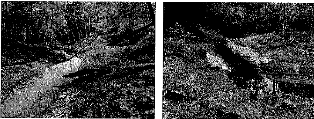
Figure 2. Example of how the restored reach is reducing sediment load downstream; left photo shows streamflow entering the restored reach, and right photo shows streamflow leaving the restored reach downstream (provided by RPBCWD).
