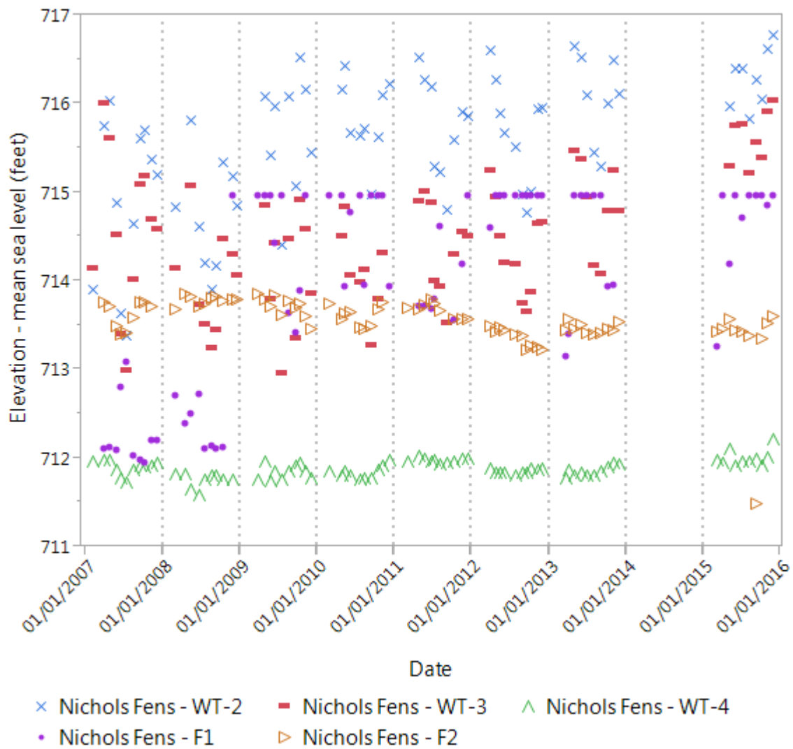
Figure 6. Water level elevation for the Nichols Fen wells (set 3 of 3), March through December, 2007-2015. At well F1, the water was often overflowing and the elevation of the top of the pipe (714.97) was recorded. See individual well graphs in Appendix 3.
