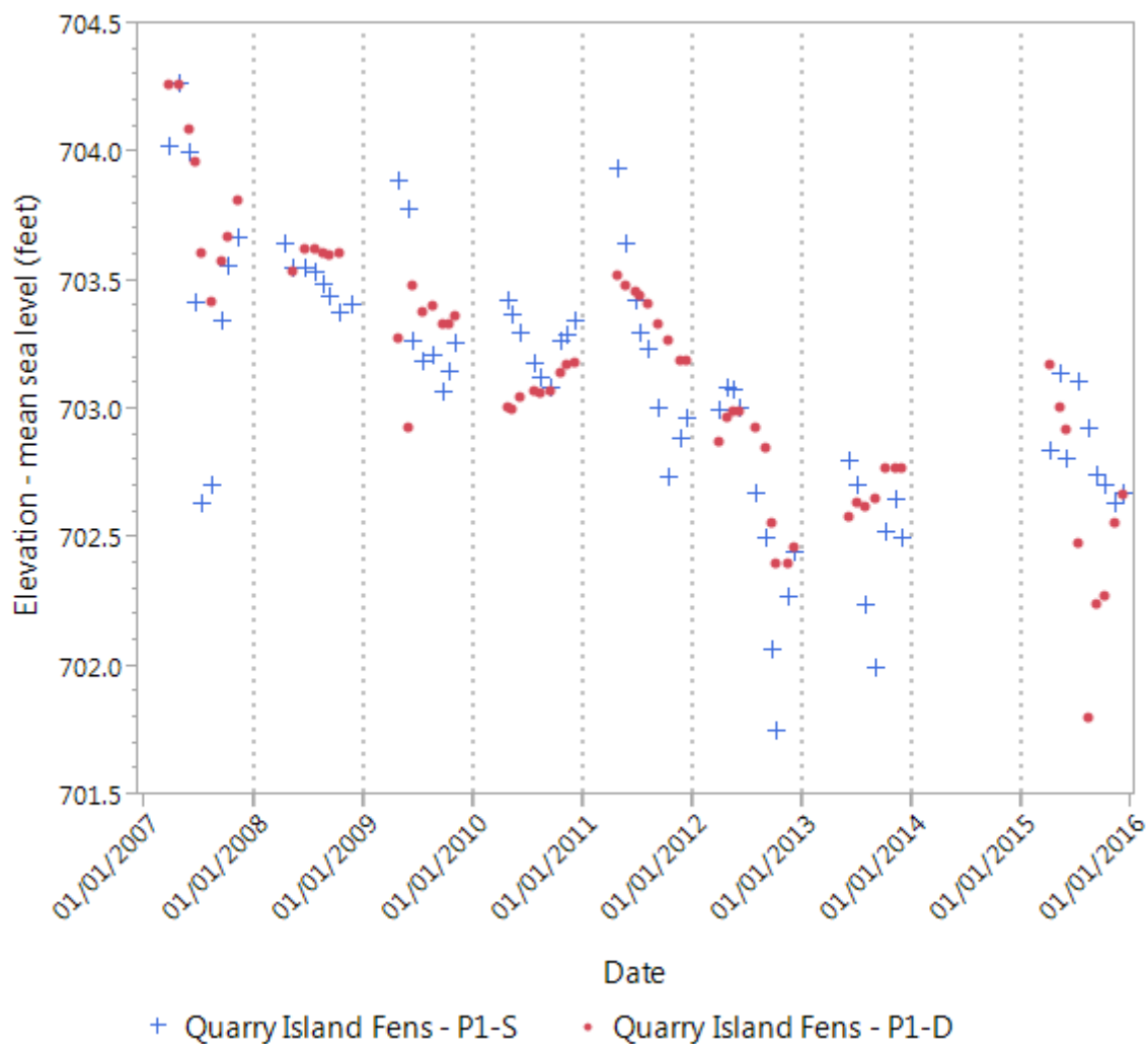
Figure 2. Water level elevation for Quarry Island Fen wells, March through December, 2007-2015.
