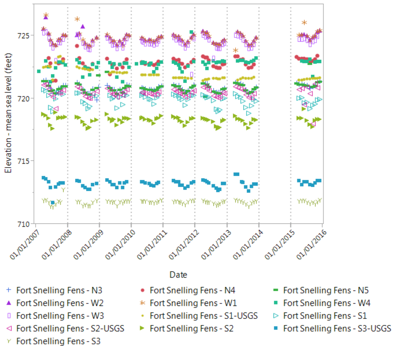
Figure 3. Water level elevation for the Fort Snelling Fen wells, March through December, 2007-2015. At well S3-USGS, when the water was overflowing, the elevation of the top of the pipe (713.97) was recorded. See individual well graphs in Appendix 3.
