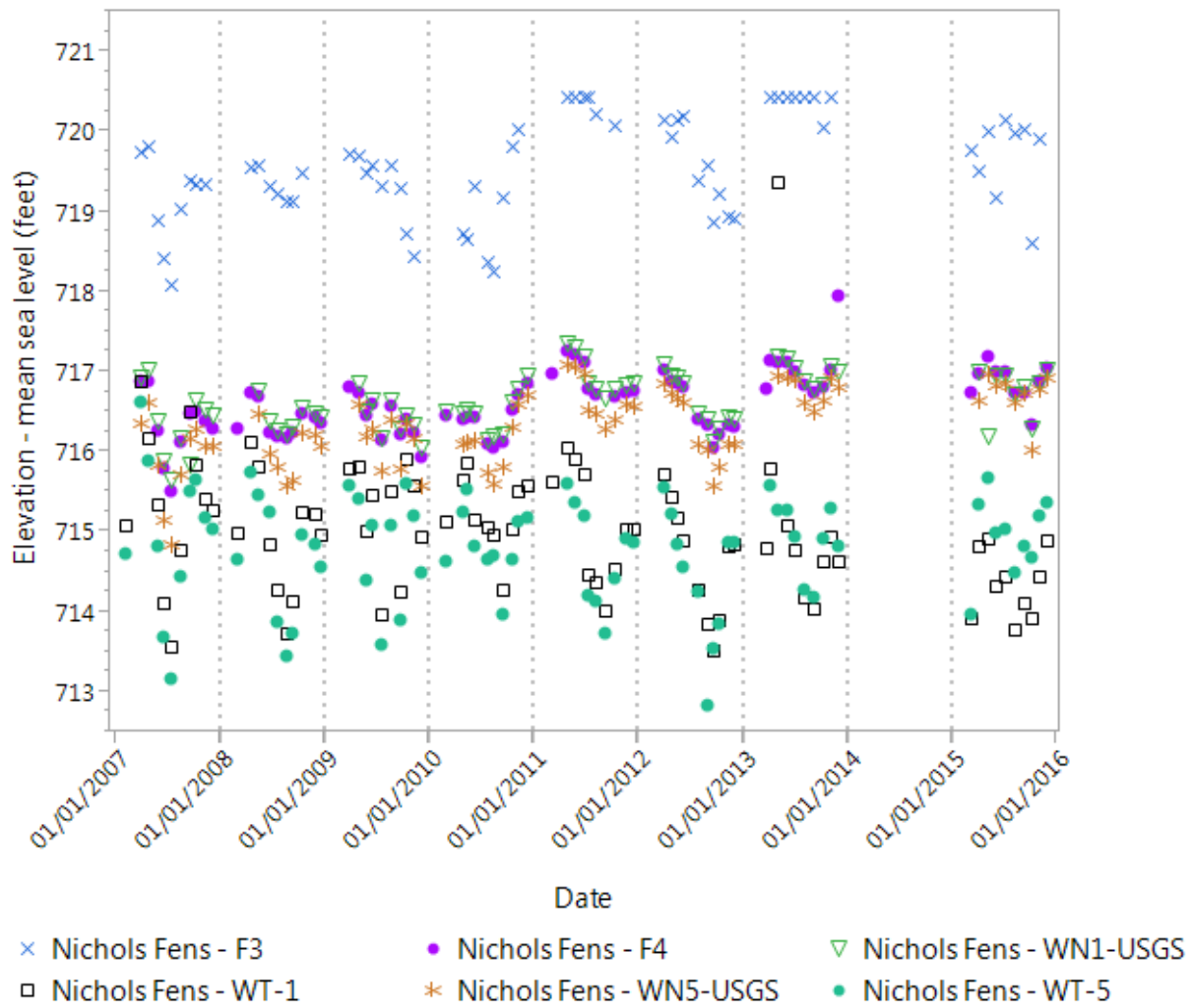
Figure 5. Water level elevation for the Nichols Fen wells (set 2 of 3), March through December, 2007-2015. At well F3 and WT-1, the water was often overflowing and the elevation of the top of the pipe (720.43 and 719.37, respectively) was recorded. See individual well graphs in Appendix 3.
