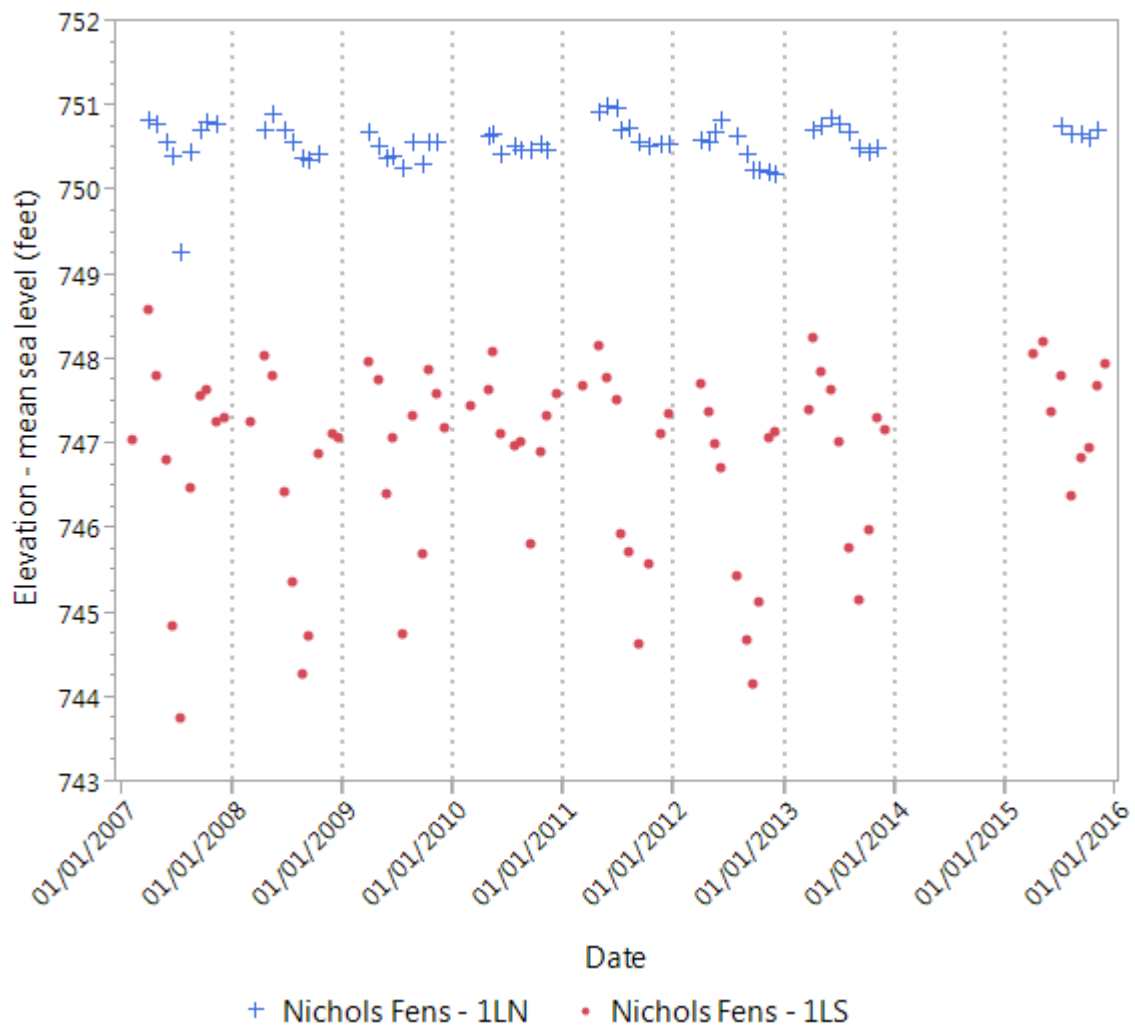
Figure 4. Water level elevation for the Nichols Fen wells (set 1 of 3), March through December, 2007-2015.
